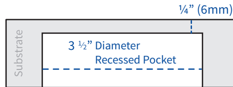
Figure 3b. The recessed hole must be 6mm from the surface
