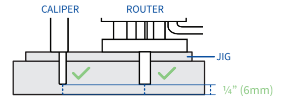
Figure 2a. Measure the table and jig thickness together.
